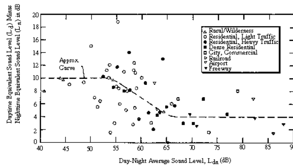
Figure A-7. Comparison of the Difference Between Day and Night Values of the Equivalent Sound Level with the Day-Night Average Sound Level, L_{dn} A-25
